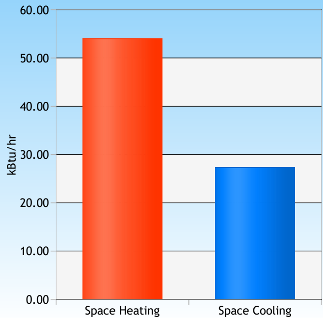
Design Loads
