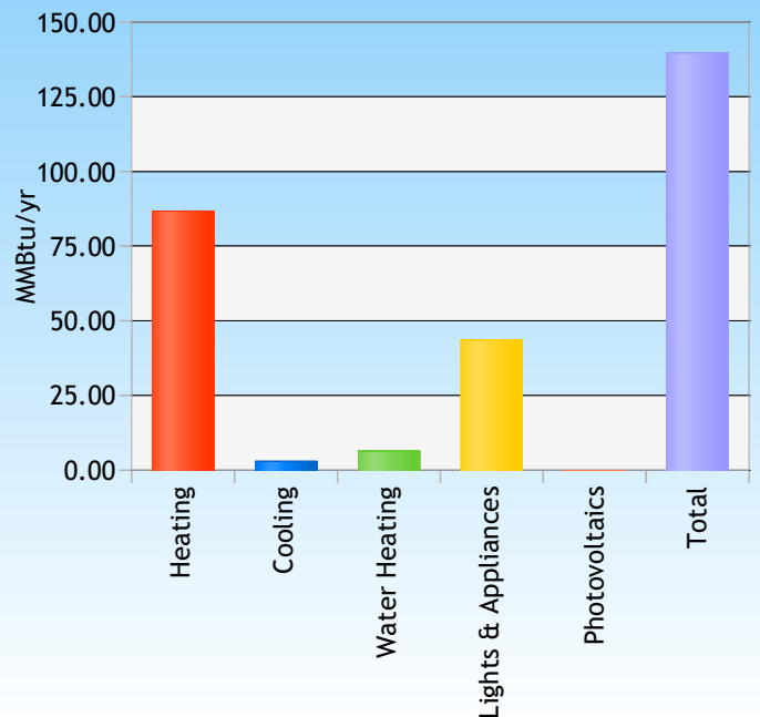
Annual Consumption
