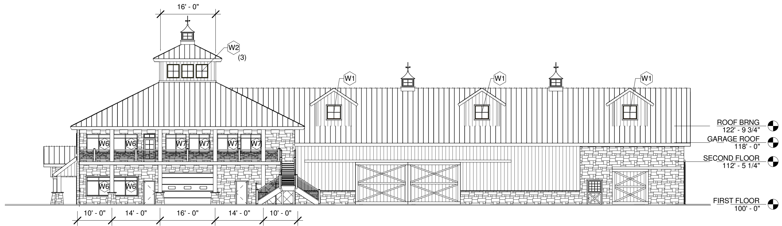
① WEST 1/16" = 1'-0"
