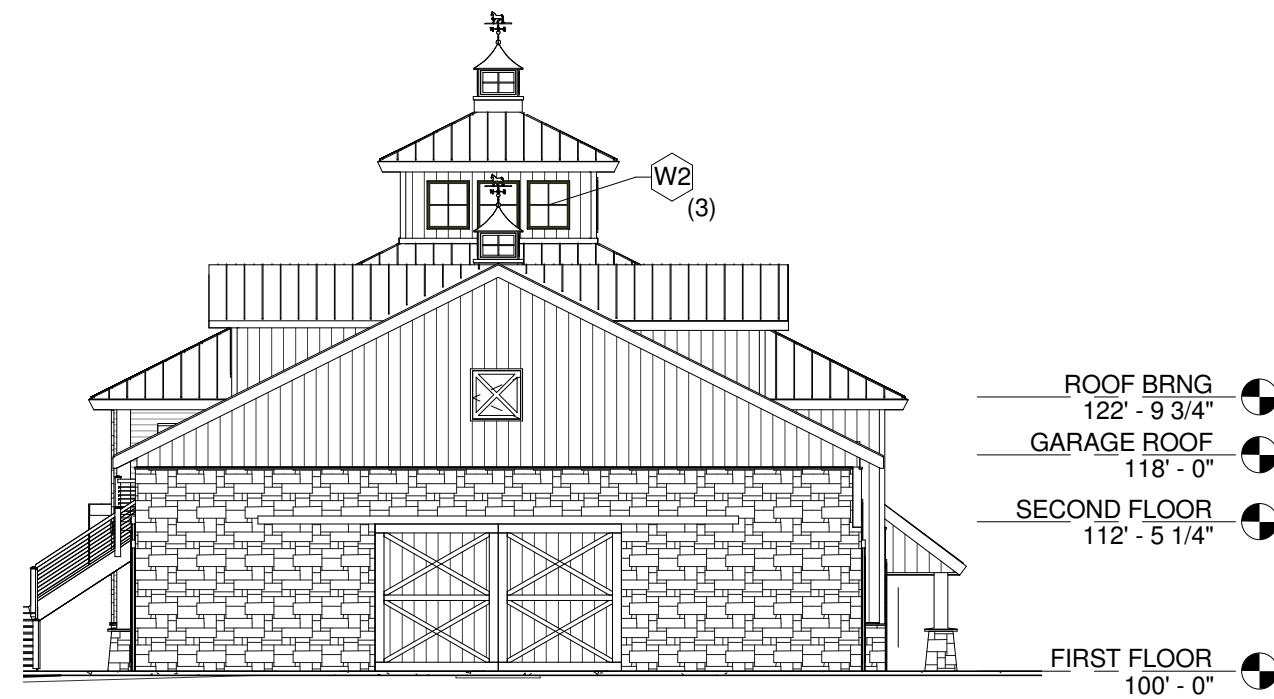
② SOUTH 1/16" = 1'-0"
