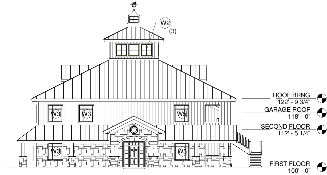
③ NORTH 1/16" = 1'-0"
